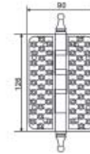
107 Door Hinge Material: Brass Finish: Rose Gold 4 Ball Bearing Size: 5" x 3.5" x 4mm Available finish: RG, CB, AB
