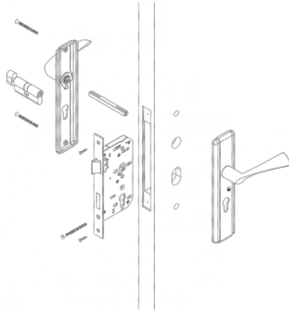
Installation diagram of lockset with plate
