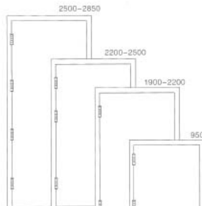
Quantity of hinges based on the door height
