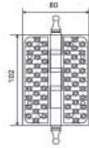
106 Door Hinge Material: Brass Finish: Rose Gold 4 Ball Bearing Size: 4" x 3" x 4mm Available finish: RG, CB, AB
