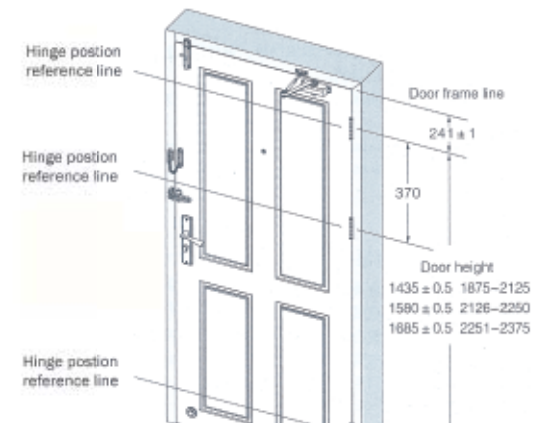
Position of hinges and other ironmongeries
