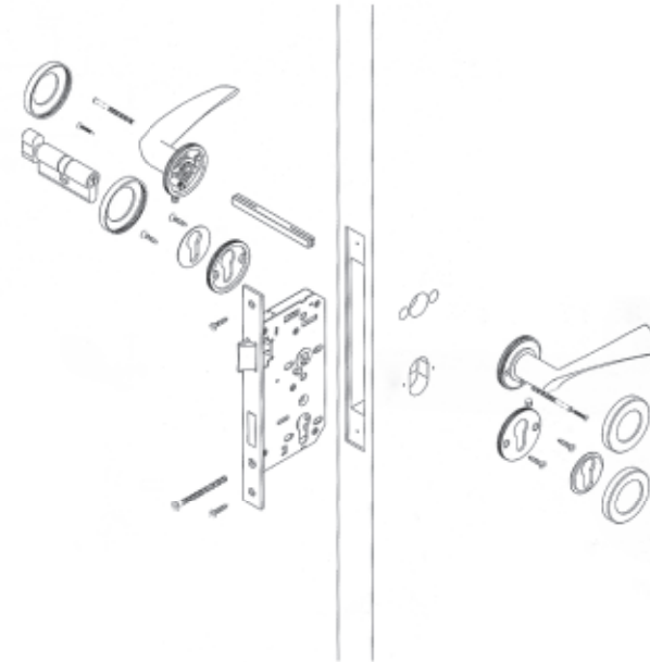
Installation diagram of lockset with rose
