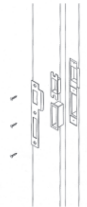
Installation diagram of lockplate
